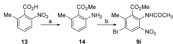
Scheme 3. (a) (i) K 2 CO 3 , MeI, acetone; (ii) 10% Pd/C, H 2 ; (b) (i) (CH 3 CO) 2 O, rt; (ii) Br 2 , AcOH; (iii) 90% HNO 3 , TFA.
