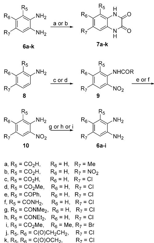
Scheme 1. (a) (CO 2 H) 2 , 2N HCl; (b) (CO 2 Et) 2 , EtOH; (c) (i) (CH 3 CO) 2 O; (ii) KNO 3 /H 2 SO 4 ; (d) (CF 3 CO) 2 O, CF 3 CO 2 H, then KNO 3 ; (e) 2N HCl; (f) K 2 CO 3 or NaOH; (g) SnCl 2 ·2H 2 O; (h) (NH 4 ) 2 S; (i) H 2 , Pd/C.
