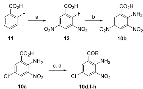
Scheme 2. (a) 90% HNO 3 , H 2 SO 4 (fuming, 15% SO 3 ), 145 °C, 73%; (b) 30% NH 4 OH, HCl, rt, 97%; (c) SOCl 2 , reflux; (d) CH 3 OH or NH 3 or HN(CH 3 ) 2 or HN(CH 2 CH 3 ) 2 , rt, 81–98%.
