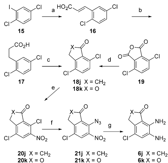
Scheme 4. (a) CH 2 =CHCO 2 H, Pd(OAc) 2 , TEA, CH 3 CN, 94%; (b) PtO 2 , H 2 , EtOAc; (c) (i) SOCl 2 ; (ii) AlCl 3 , CS 2 , 71%; (d) NaBH 4 , DMF, rt, 75%; (e) 90% HNO 3 , 43% or KNO 3 , H 2 SO 4 , 86%; (f) NaN 3 , acetone, H 2 O, 75%; (g) 10% Pd/C, H 2 , EtOAc.
